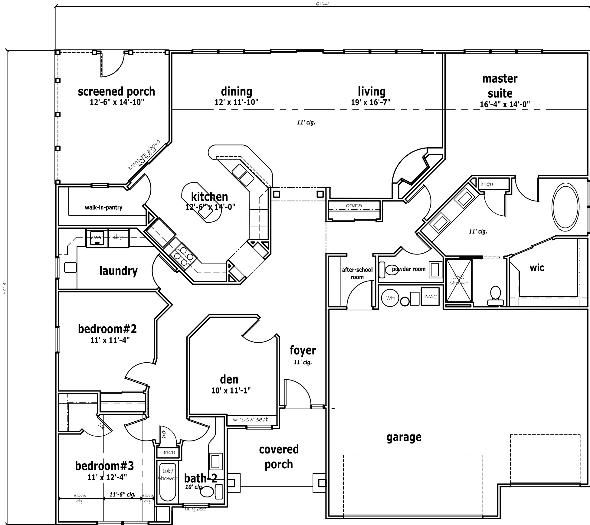
MAIN LEVEL FLOOR PLAN 2,230 sq ft
